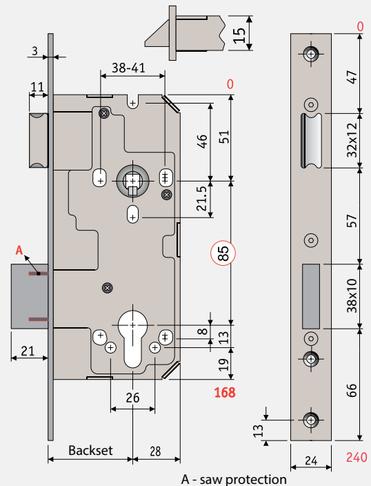
A - saw protection
